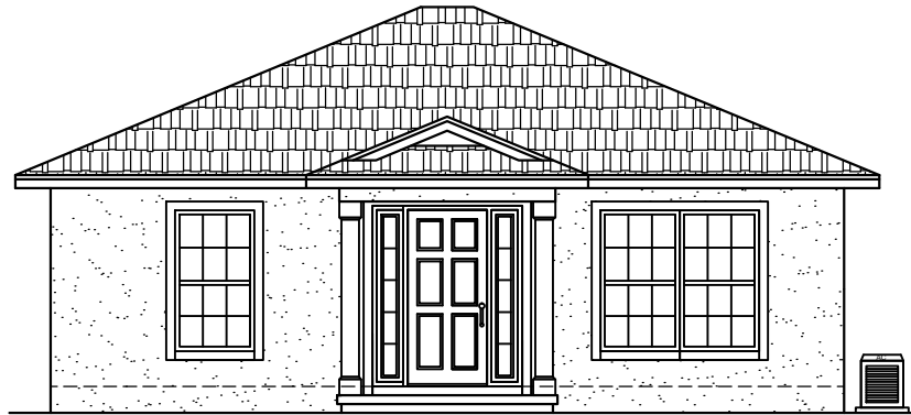
THE NOBLETON (30'-0"W X 32'-0"D) © COPYRIGHT TRINITY DRAFTING LLC
