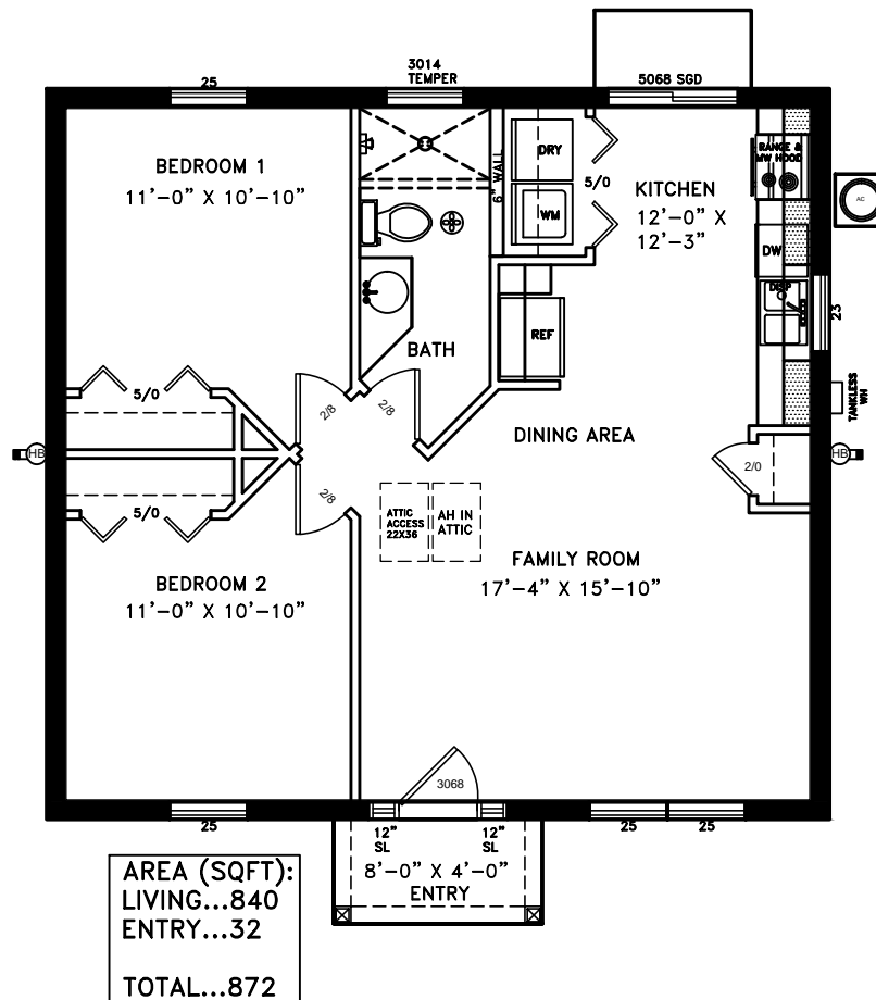
THE NOBLETON (30'-0"W X 32'-0"D) © COPYRIGHT TRINITY DRAFTING LLC
